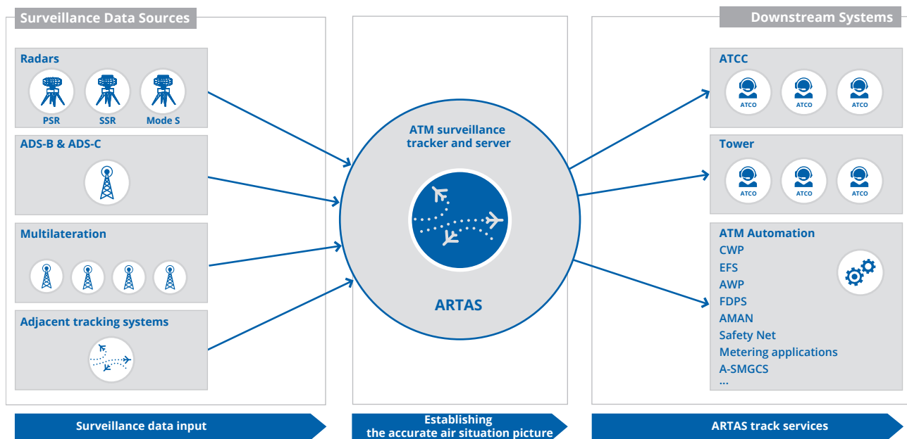
Figure 2: Schematic of ARTAS inputs and outputs
